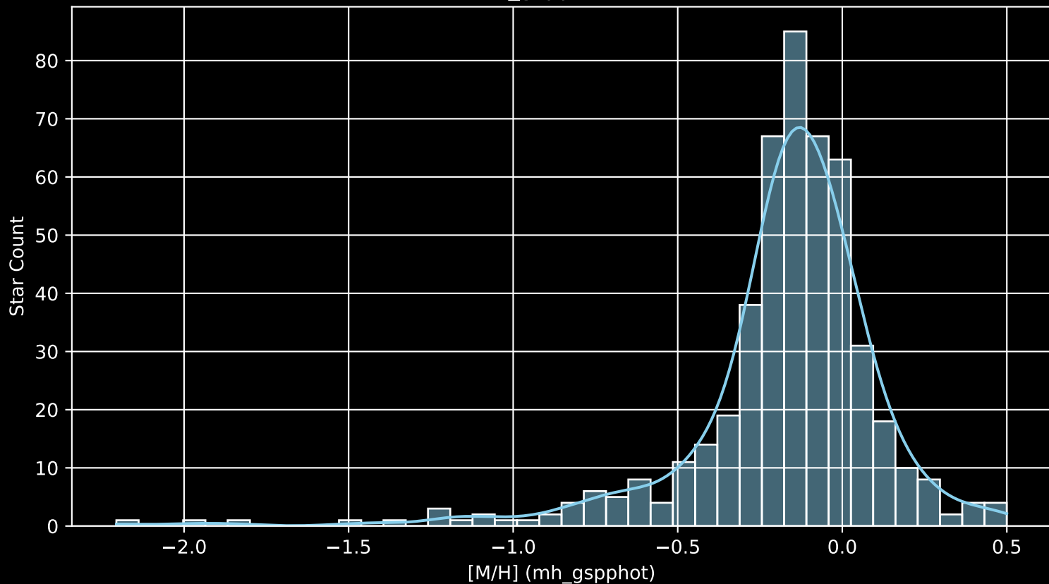
APOGEE DR17 Field: [165+04 [M/H] (mh_gspphot) (n= 483)
