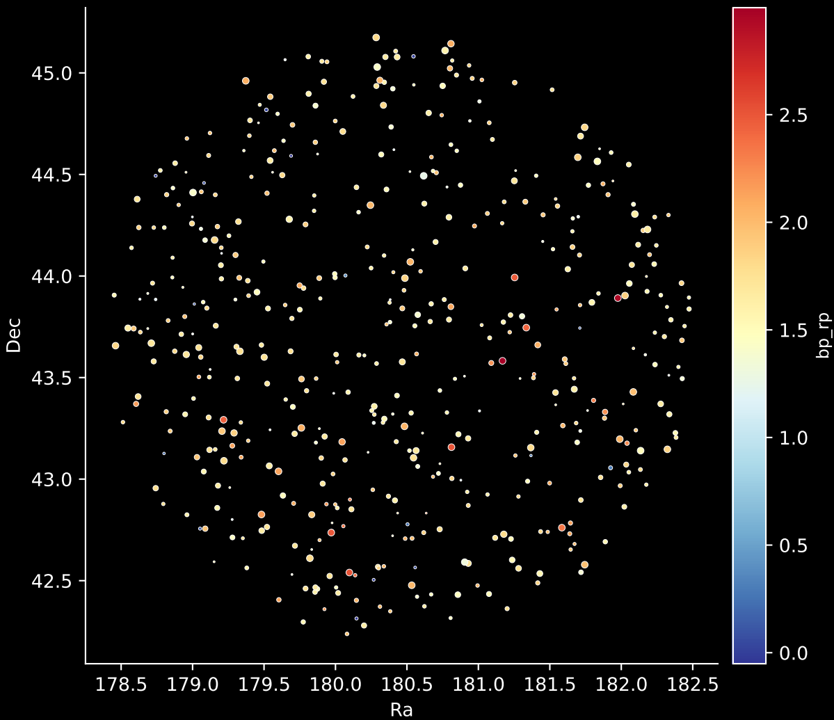
APOGEE DR17 Field: [165+04] Stars: 488
