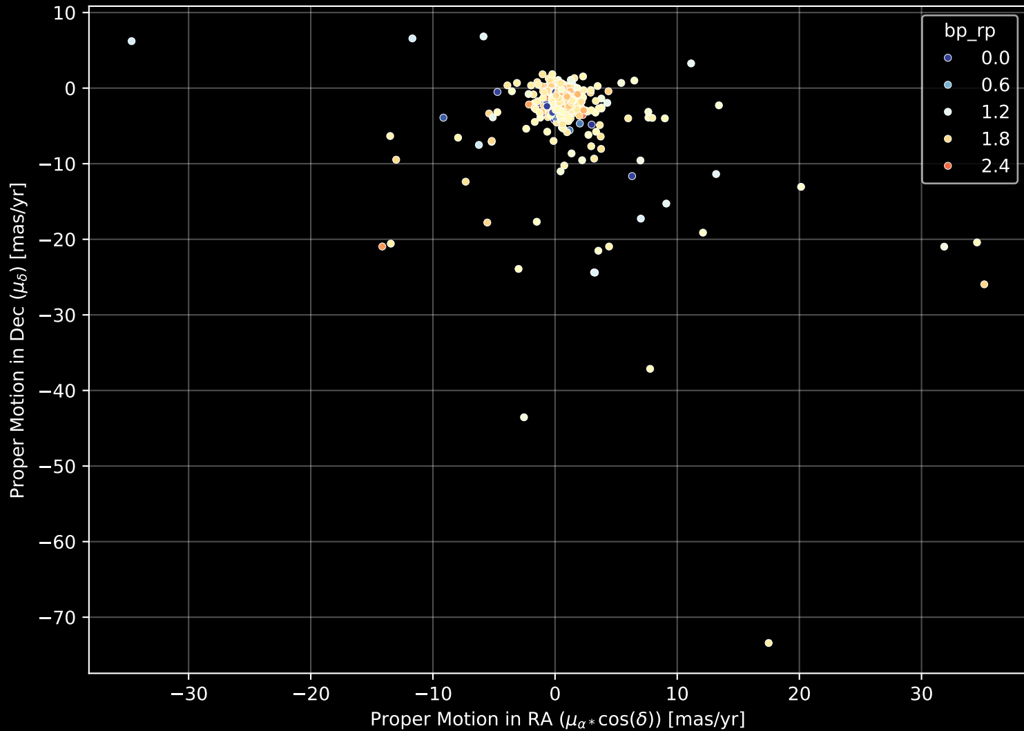
APOGEE DR17 Field: [165+04] Proper Motion Diagram (n= 488)
