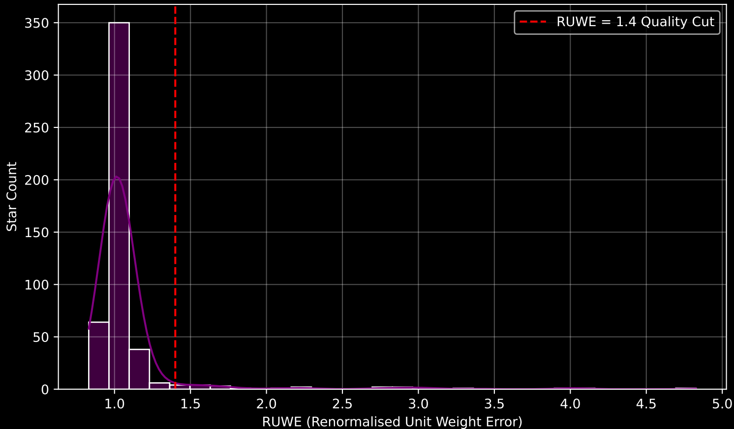
GAPOGEE DR17 Field [165+04] RUWE Distribution (n= 482)
