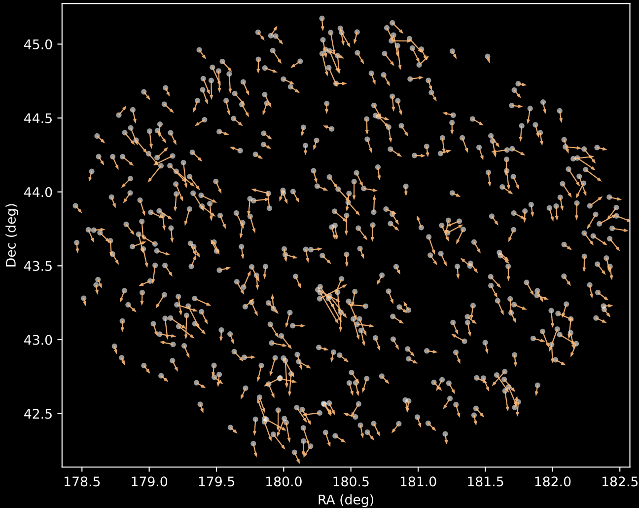
APOGEE DR17 Cluster 3 Proper Motion Vectors (n=443)
