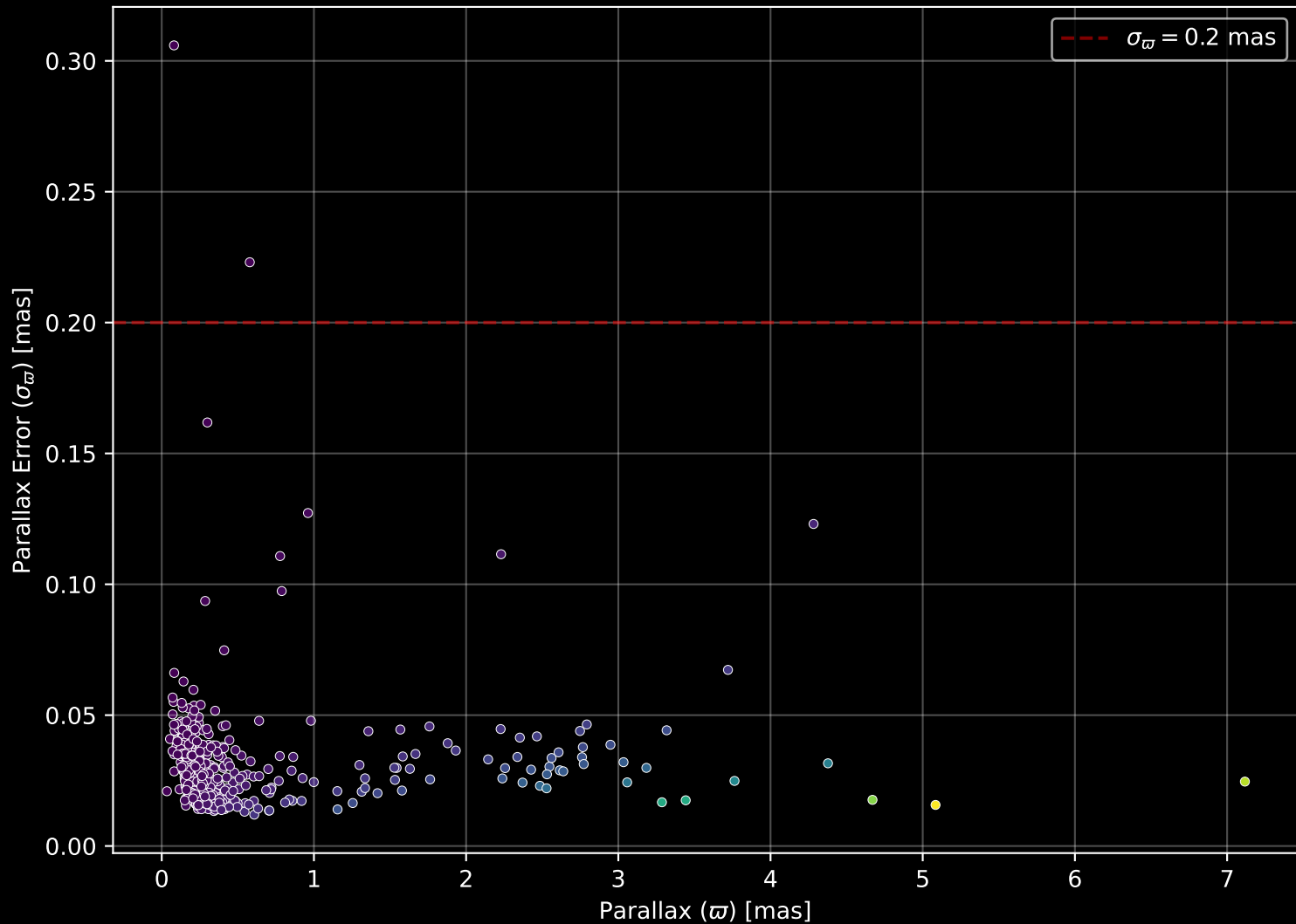
APOGEE DR17 Field: [165+04] Parallax Quality (n= 488)
